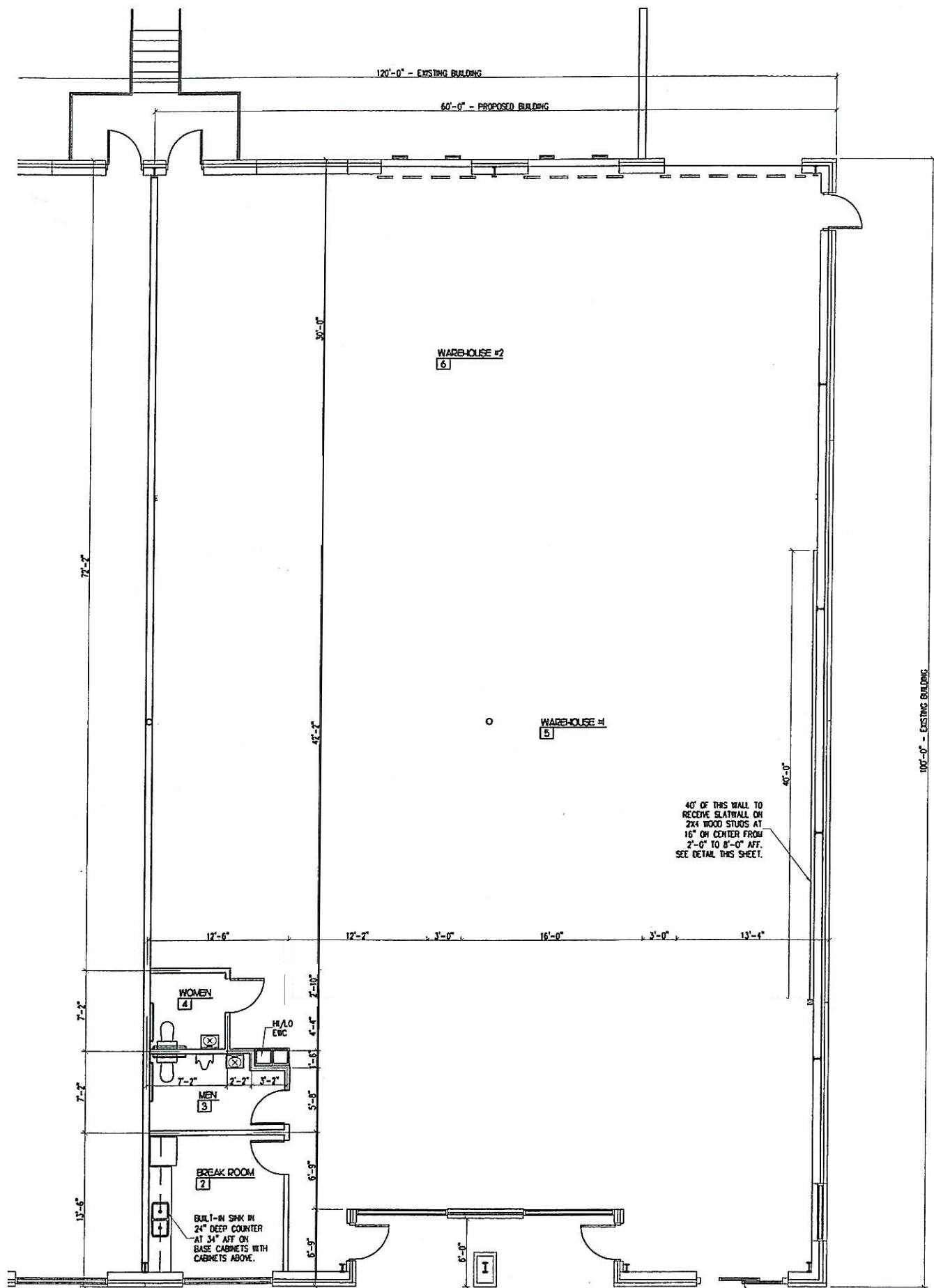
PRELIMINARY INTERIOR UPFIT FLOOR PLAN SCALE: 3/16" = 1'-0"
